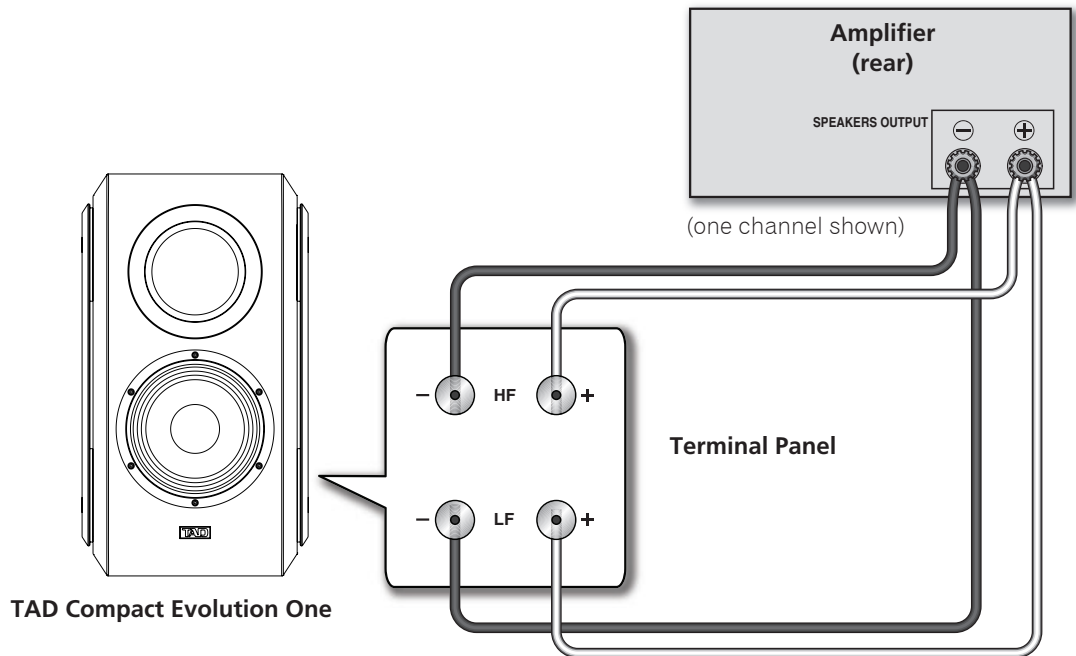
Figure 3. Connecting a TAD Compact Evolution One speaker in a bi-wired system
