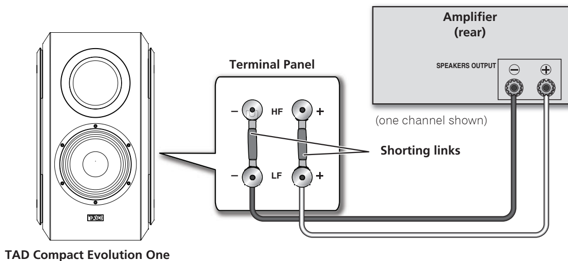
Figure 2. Connecting a TAD Compact Evolution One speaker in a single-wired system
