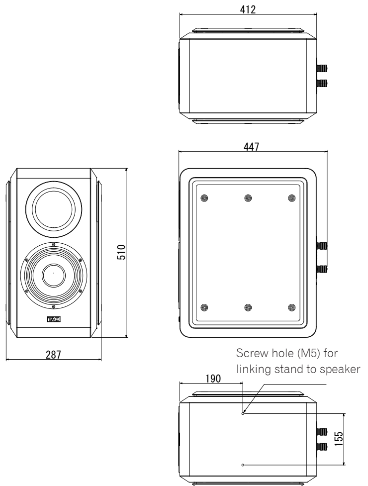
Figure 6. Overall dimensions of the TAD Compact Evolution One speaker system
